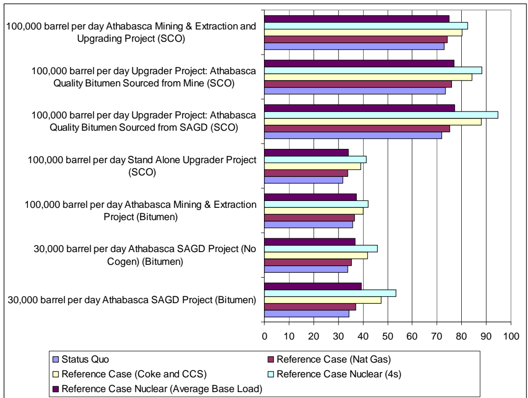
Figure 4.2 Summary of Supply Costs $/bbl of Bitumen and SCO (where applicable)
